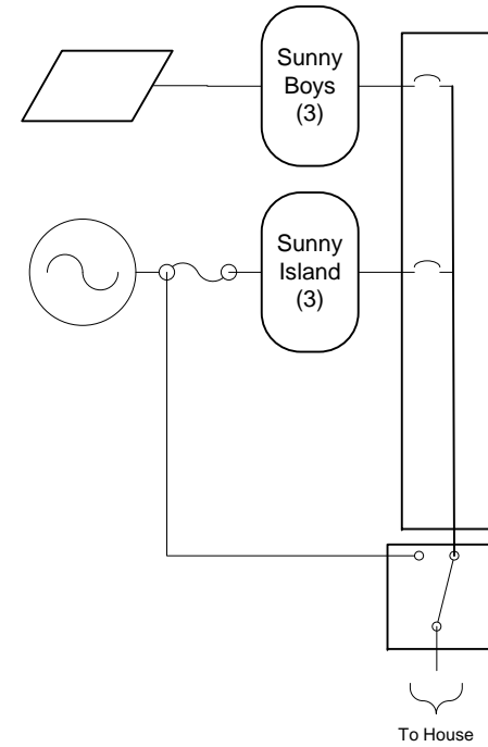
PLAN B: EXTERNAL INTERLOCK
