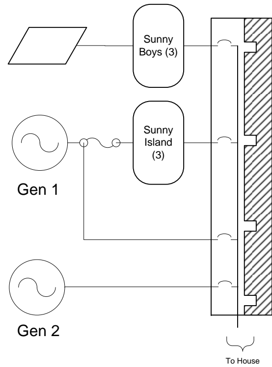
PLAN A: BREAKER INTERLOCK (Chosen method)
