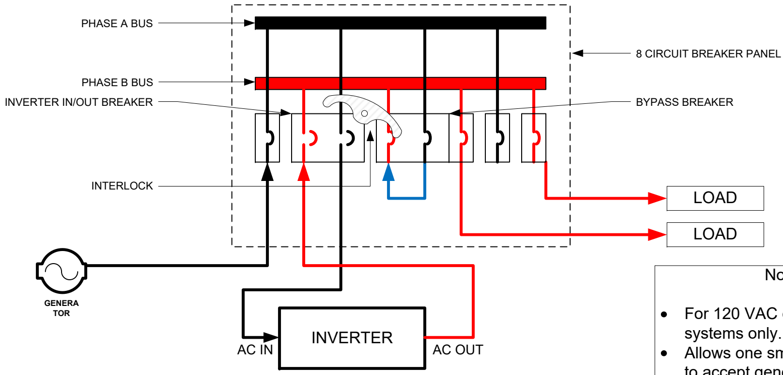
BLOCK DIAGRAM (Shown in bypass mode)
